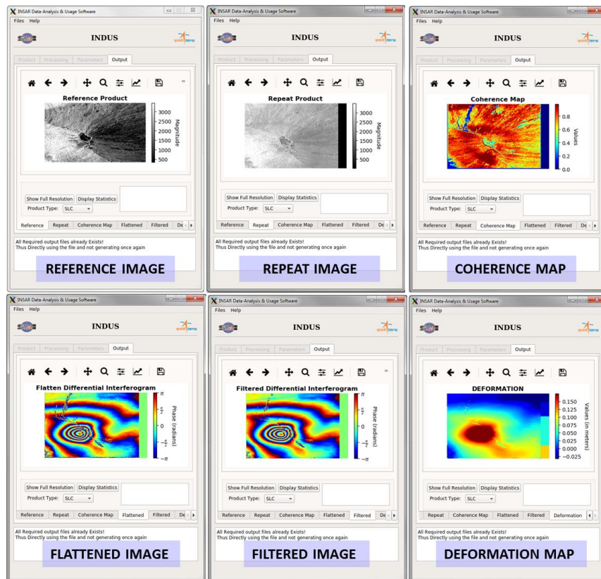
Figure 5 : Output Images of the Interferometric Processing in Range Doppler Domain
