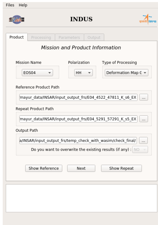
Figure 1 : Interferometric SAR Data Analysis & Usage Software (INDUS) GUI Home Panel
